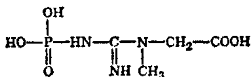
Phosphocreatine (Source: Merck Index)
