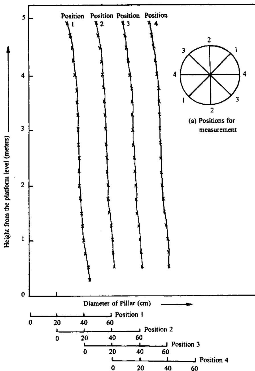
Fig. 3: Variation of diameter of the Iron Pillar with height (Courtesy: Bindal et al , National Physical Laboratory, New Delhi, 1989)
