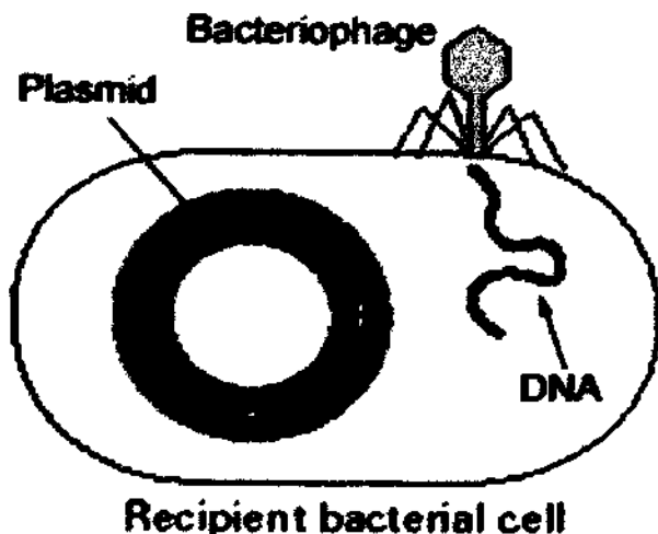
Bacteriophage inserting its DNA into bacterial cell.
