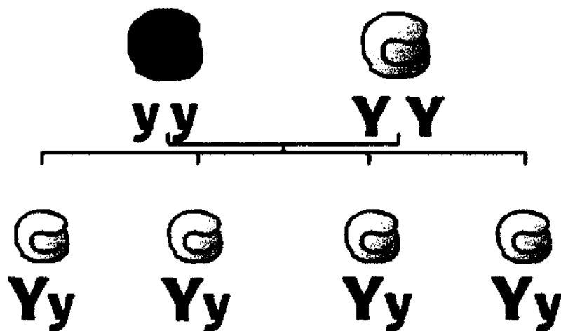
Crossing of plants bearing green seeds with plants bearing yellow seeds produced only yellow seeds
