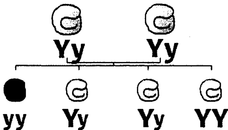
Crossing of yellow seed hybrids with the same variety produced green seeds in the ratio 1:3
