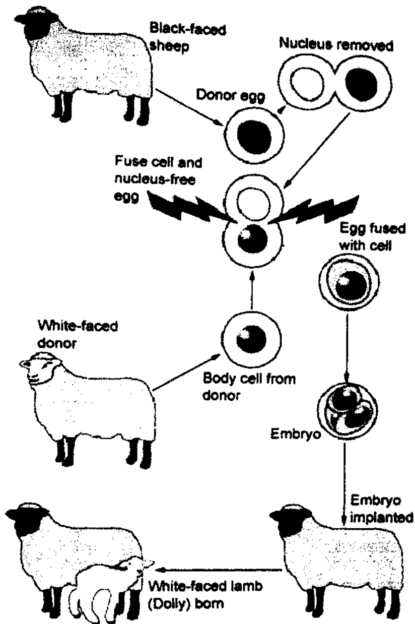
Steps used to clone Dolly
