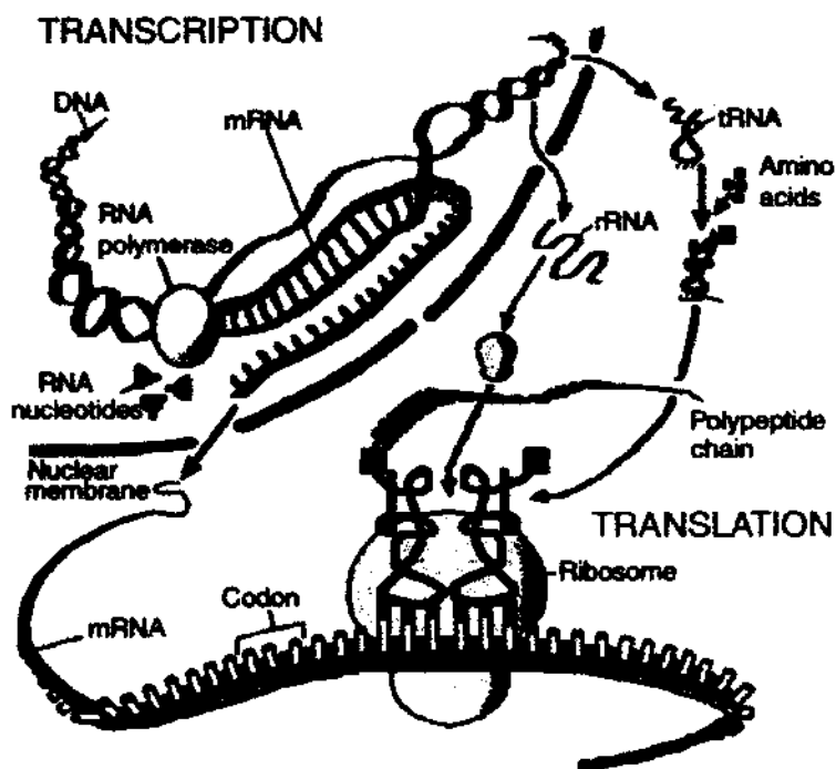
The steps in protein synthesis
