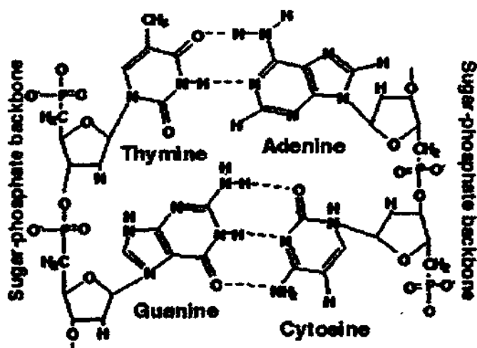
Base pairing between guanine-cytosine and adenine-thymine
