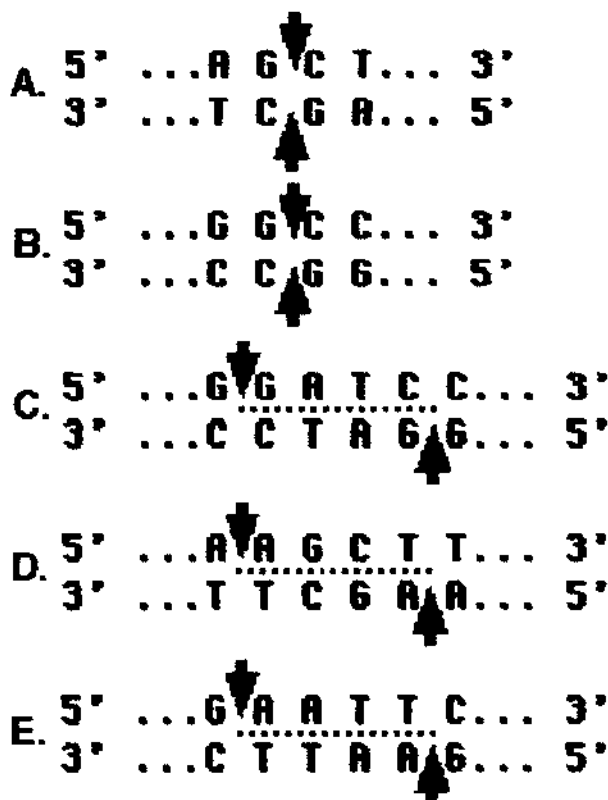
How restriction enzymes cut DNA at specific locations
