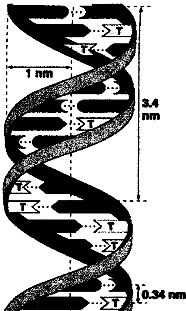
The DNA double helix
