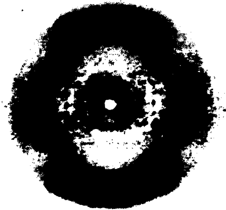
X-ray diffraction pattern of DNA
