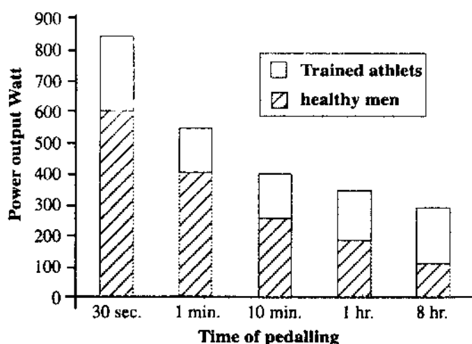
Effect of duration on the pedalling power output. The graph shows that the power output level in short bursts could be upto six times that in long runs. Comfortable level for routine bicycling is taken at 60 W.
