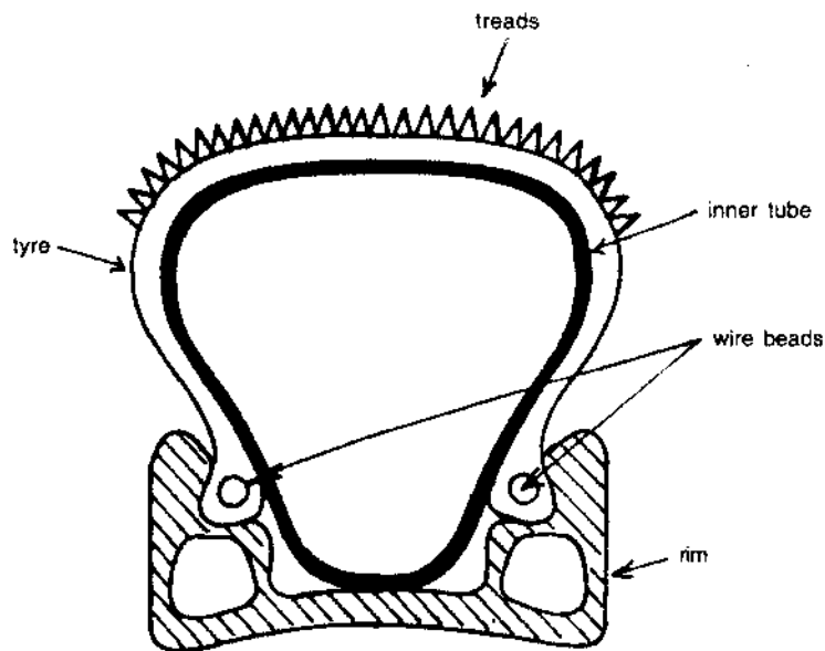
Cross-section of a rim and a conventional wire-bead tyre. Beads are tensioned and keep the tyre in place.
