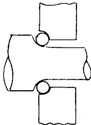
Schematic of a typical ball bearing in a bicycle. The shaft constitutes the hardened 'cone' and the frame has the 'cup'. The balls run between the cup and the cone.
