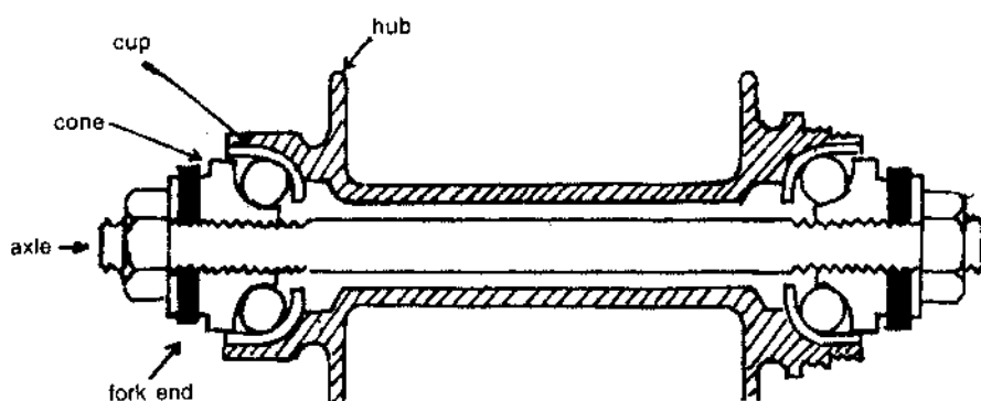
A section of the front hub bearing
