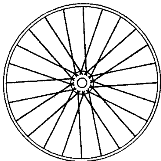
Spokes tangent at the hub is the lightest solution for a wheel. It is restrained in all the six degrees of freedom.
