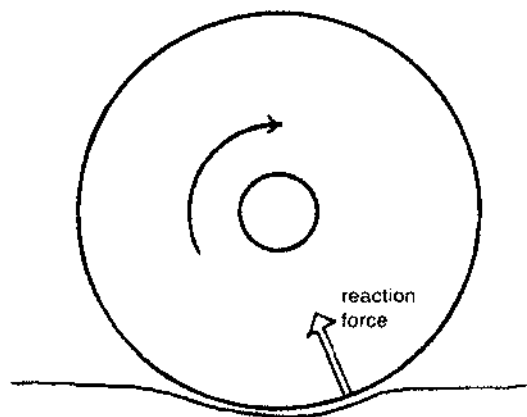
When a soft tyre rolls on a soft ground, both the tyre and the ground deform. The deformed ground sets up a reaction force so directed that it resists the motion. Similarly, the deformation of tyre, too, does not permit smooth rolling.
