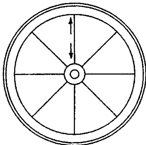
The load applied at the hub is borne in compression by the stout spokes of a cart wheel, but in tension in thin wire spokes.
