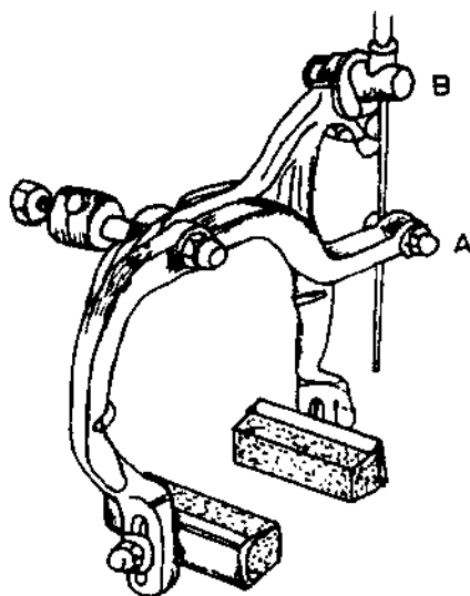
Caliper brakes operate against the sides of the rim. They are operated by the pull of the brake wire through an outer casing. The outer sleeve is attached at A and the inner cable at B.
