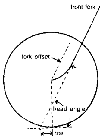
Front fork geometry. The variables that affect the stability of the bicycle.
