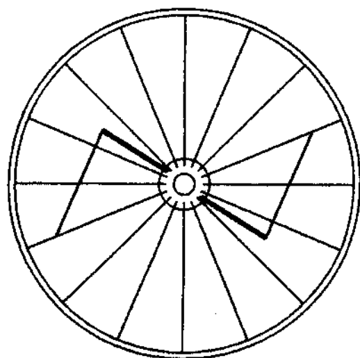
The earlier tensioned-wire spokes ran straight in to the centre of the wheel. These spokes could take the vertical load at the hub but couldn't transmit the torque at the hub to the rim. A couple of rigid bars with their own tensioned spokes were added for the purpose.
