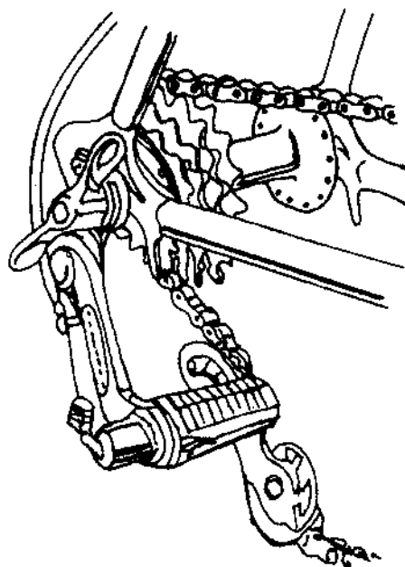
An inner-cable-through-outer-sleeve pulls the derailleur to a side, derailing the chain from one sprocket to another. The spring loaded idle roller takes up the slack of the chain.
