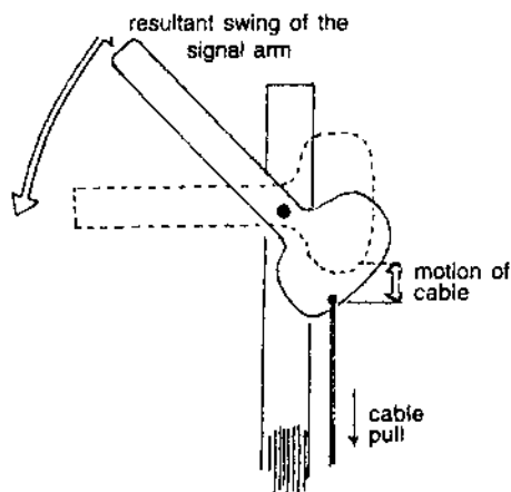
The principle of levers. By keeping 'effort' arm small one can move the 'load' through a larger distance. This is inverse of the usual situation where effort arm is made larger to overcome a larger load by a smaller effort.
