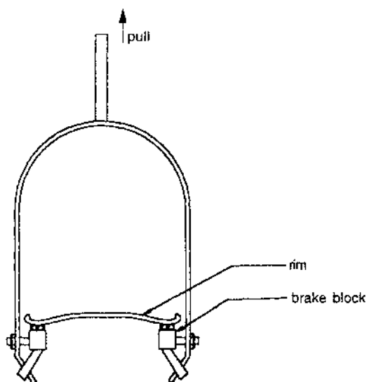
The stirrup brakes, still common in Indian bicycles, operate on the underside of the rim. The operating mechanism of these brakes is quite unreliable. These also need far too frequent adjustments.
