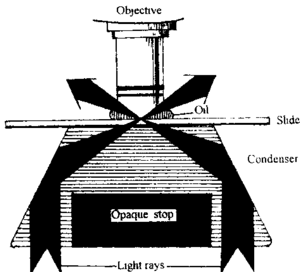
Fig. 36: Showing path of rays through the condenser in a dark ground microscope
