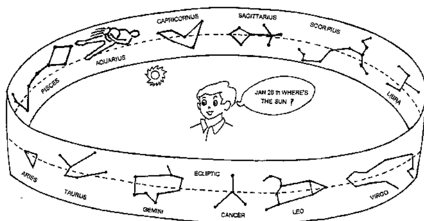
Fig. 8 The Zodiacal Belt
