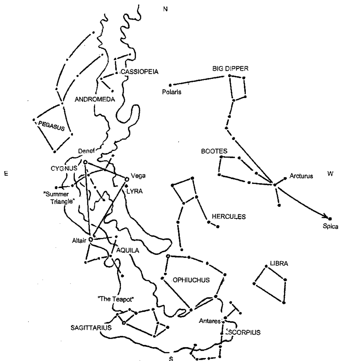
Fig. 32 The Stars of Summer
