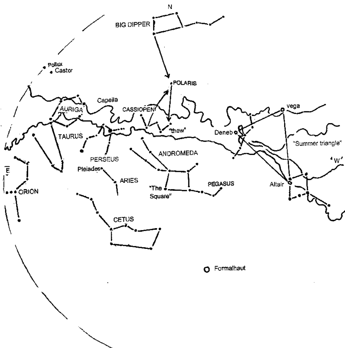
Fig. 34 The Stars of Autumn
