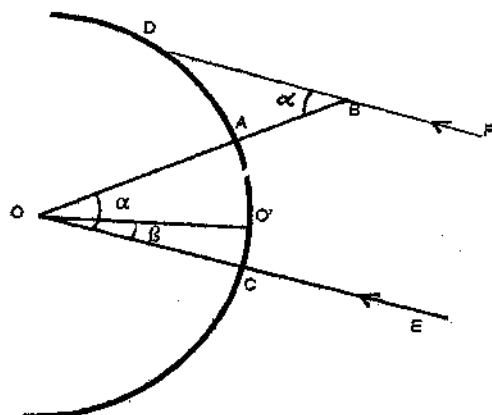
Fig. 55 C. Winter in the Southern Hemisphere
