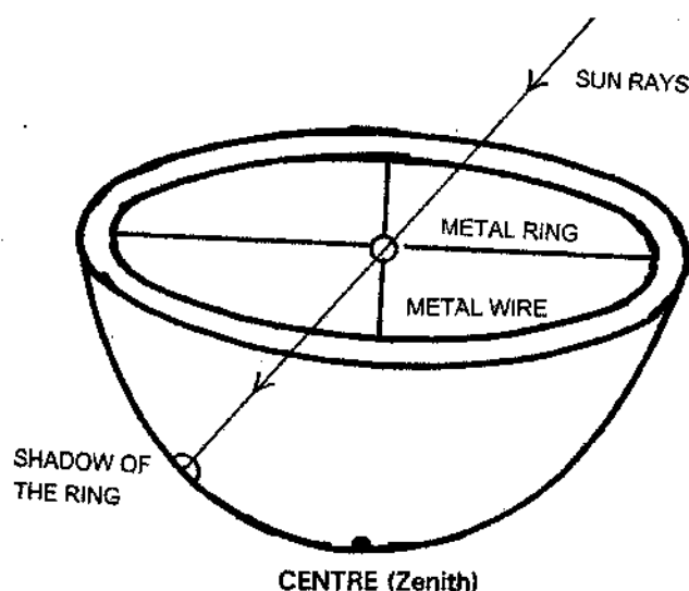
Fig. 48. The Hemispherical Bowl Instrument
