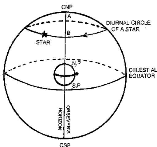
Fig. 5 Star Appears to Rise At A and Set At B
