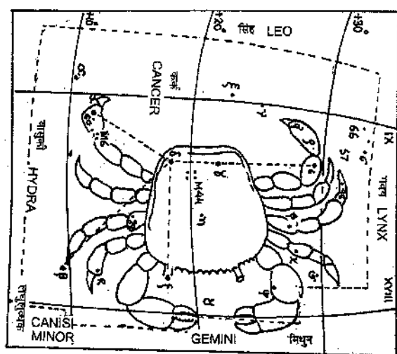
Fig. 13 Cancer
