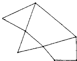
Fig. 1 Sagittarius Constellation - Teapot
