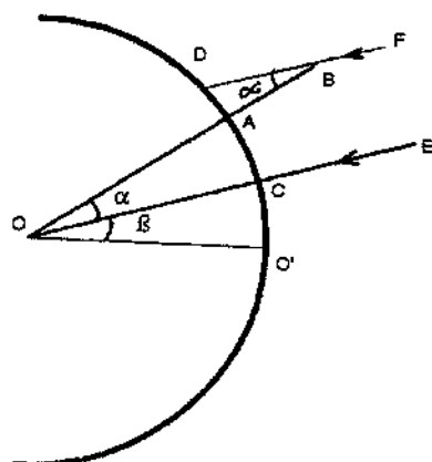
Fig. 55 b. Summer In the Northern Hemisphere
