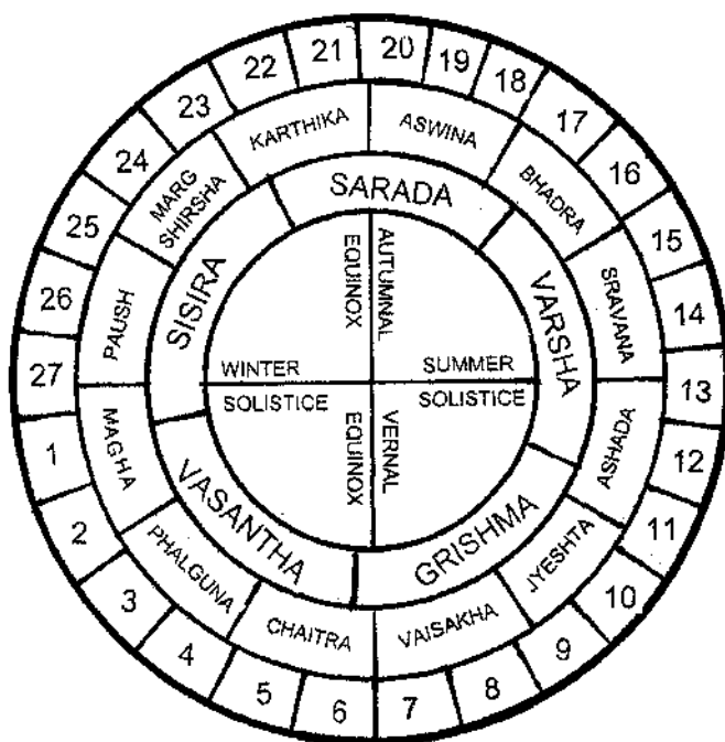
Fig. 41 The Lunar Calendar
