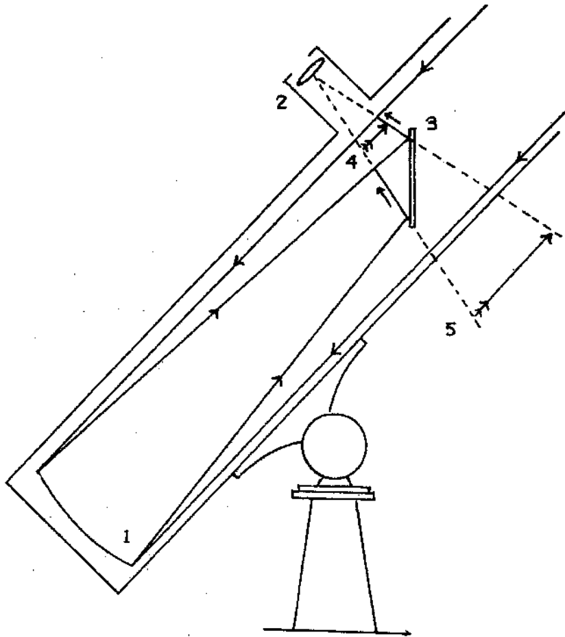
Fig. 37 Reflector Telescope
