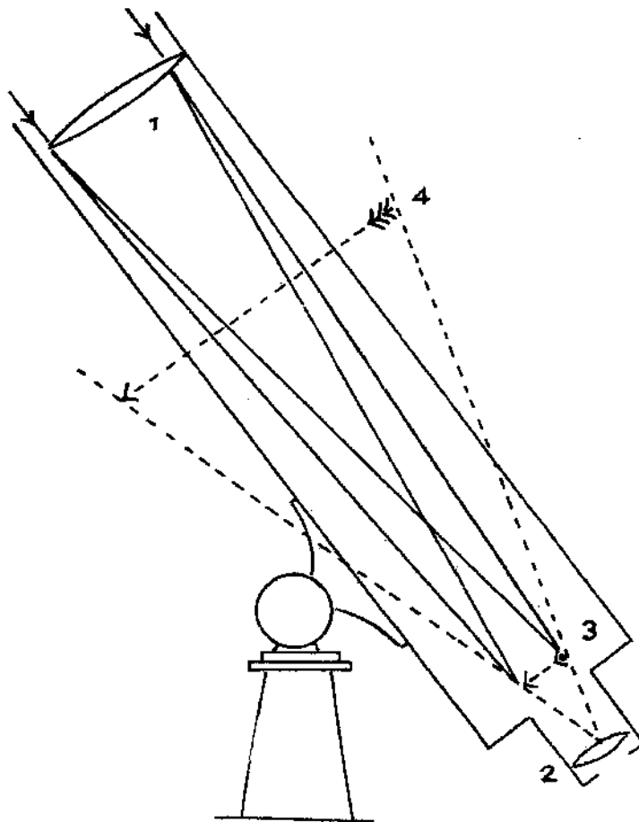
Fig. 38 Refractor Telescope
